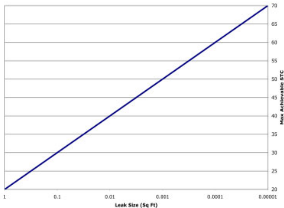
Maximum Achievable STC Rating with an Acoustical Leak in a 100 Square Foot Wall
