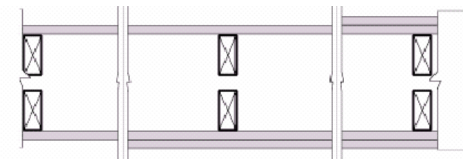
Figure 3: Double Stud Construction
